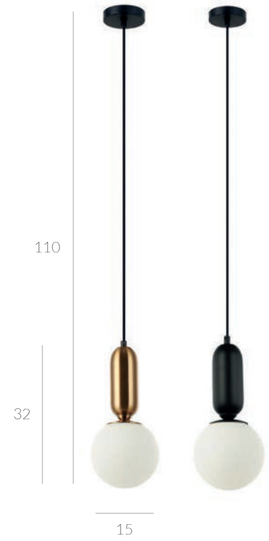
● PND-02340-1S-BRO ● PND-02340-1S-BK 💡 E27 1x40W
