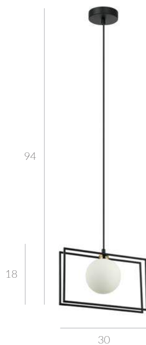
PND-55423-1-BK G9 1x25W
