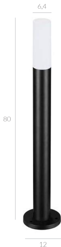
OFL-2764-S 💡 E27 1x20W 🛡️ IP54
