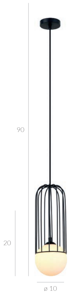
● MDM-4002/1 BK ● MDM-4002/1 GD ⚡ E27 1x40W
