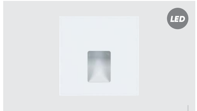
70421 Step light Vix ↔87mm ↓87mm ↗35mm
