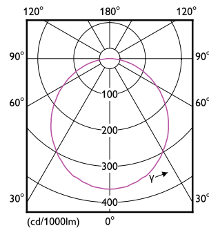
Downlight 59466 MESON 150 40K WH Recessed-LDD
